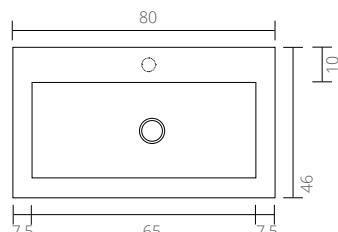
80 cm - 0 / 1 faucet hole
