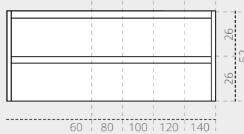
Base cabinet with 2 symmetrical drawers with recessed fronts 60 / 80 / 100 / 120 / 140 x 46 x 52 cm
