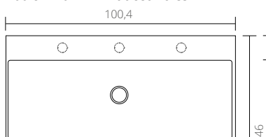
100 cm - 0 / 1 / 2 faucet holes
