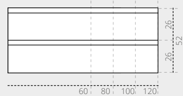
Base cabinet with 2 symmetrical drawers with overlay fronts 60 / 80 / 100 / 120 x 46 x 52 cm
