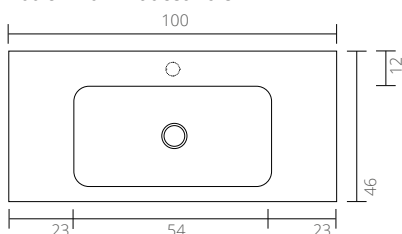
100 cm - 0 / 1 faucet hole
