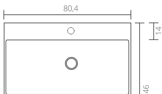
80 cm - 0 / 1 faucet hole
