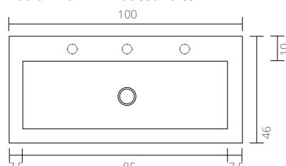
100 cm - 0 / 1 / 2 faucet holes
