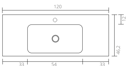
120 cm - 0 / 2 faucet holes
