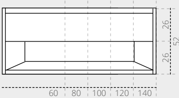
Base cabinet with 1 drawer, an open shelf and recessed front 60 / 80 / 100 / 120 / 140 x 46 x 52 cm
